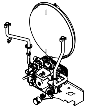
Pipework
